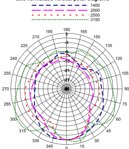
axis normalized vertical polar diagrams
