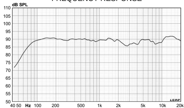
FREQUENCY RESPONSE
