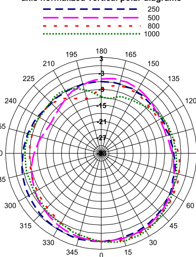
axis normalized vertical polar diagrams
